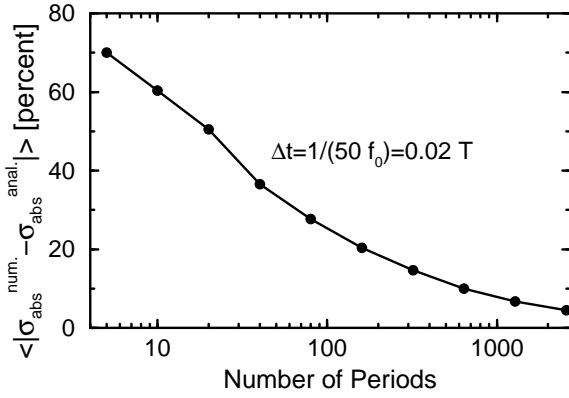
Fig. 3. Deviation of numerical absolute rms jitter from analytical result (17). The numerical value was obtained by averaging a large number of Ornstein-Uhlenbeck process realizations generated by (10).
