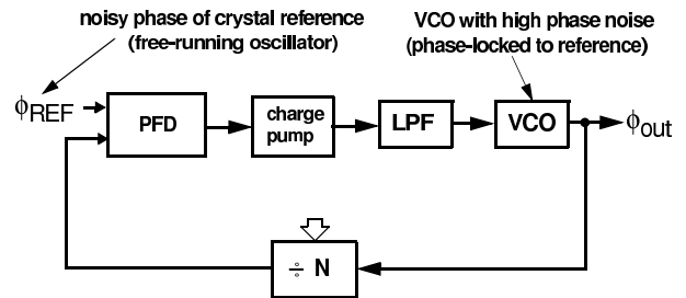
Fig. 1. Schematic view of a charge-pump PLL. The noisy VCO output is divided by N and phase-locked to a relatively clean reference to define the output frequency and to clean the VCO phase noise spectrum.
