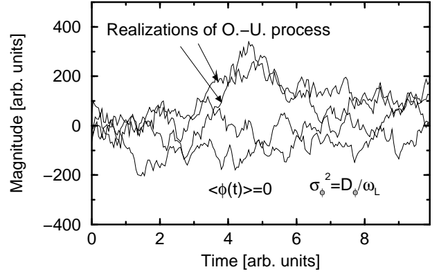
Fig. 2. Four realizations of the Ornstein-Uhlenbeck process generated by (10).
