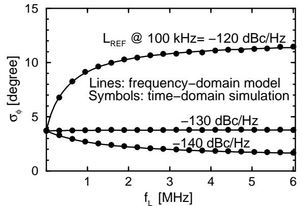
Fig. 4. RMS phase error after correction of common phase error from frequency domain model (19) and from time-domain simulation as a function of the loop bandwidth.
